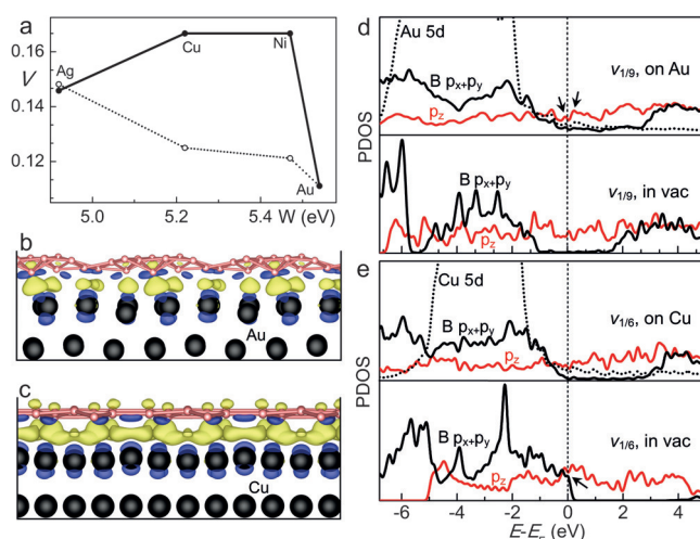
Figure 3. Mechanism of metal dependence of 2D B structures.
